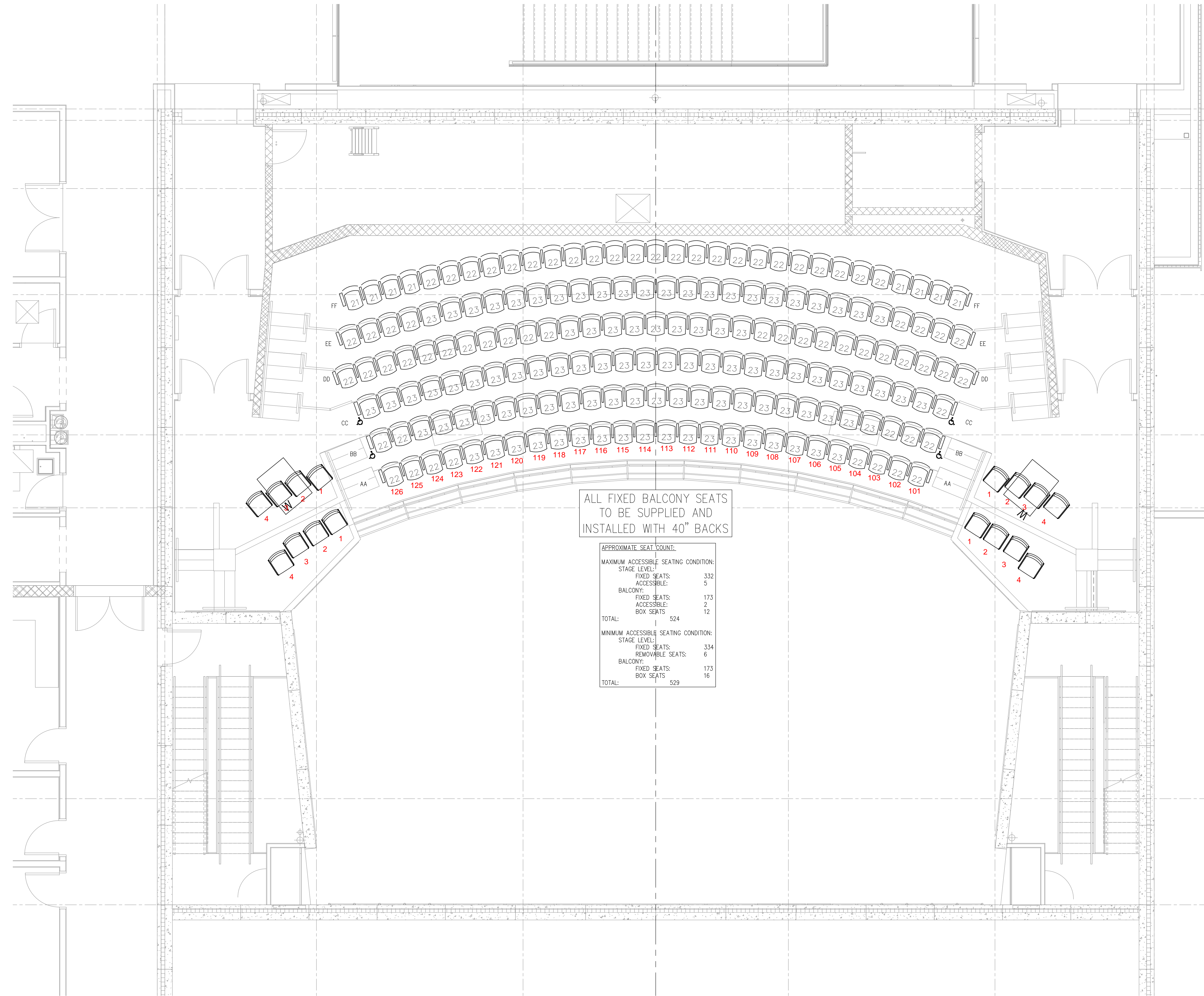
1 PLAN - BALCONY LEVEL SEATING LAYOUT SCALE: 1/4" = 1'-0"
