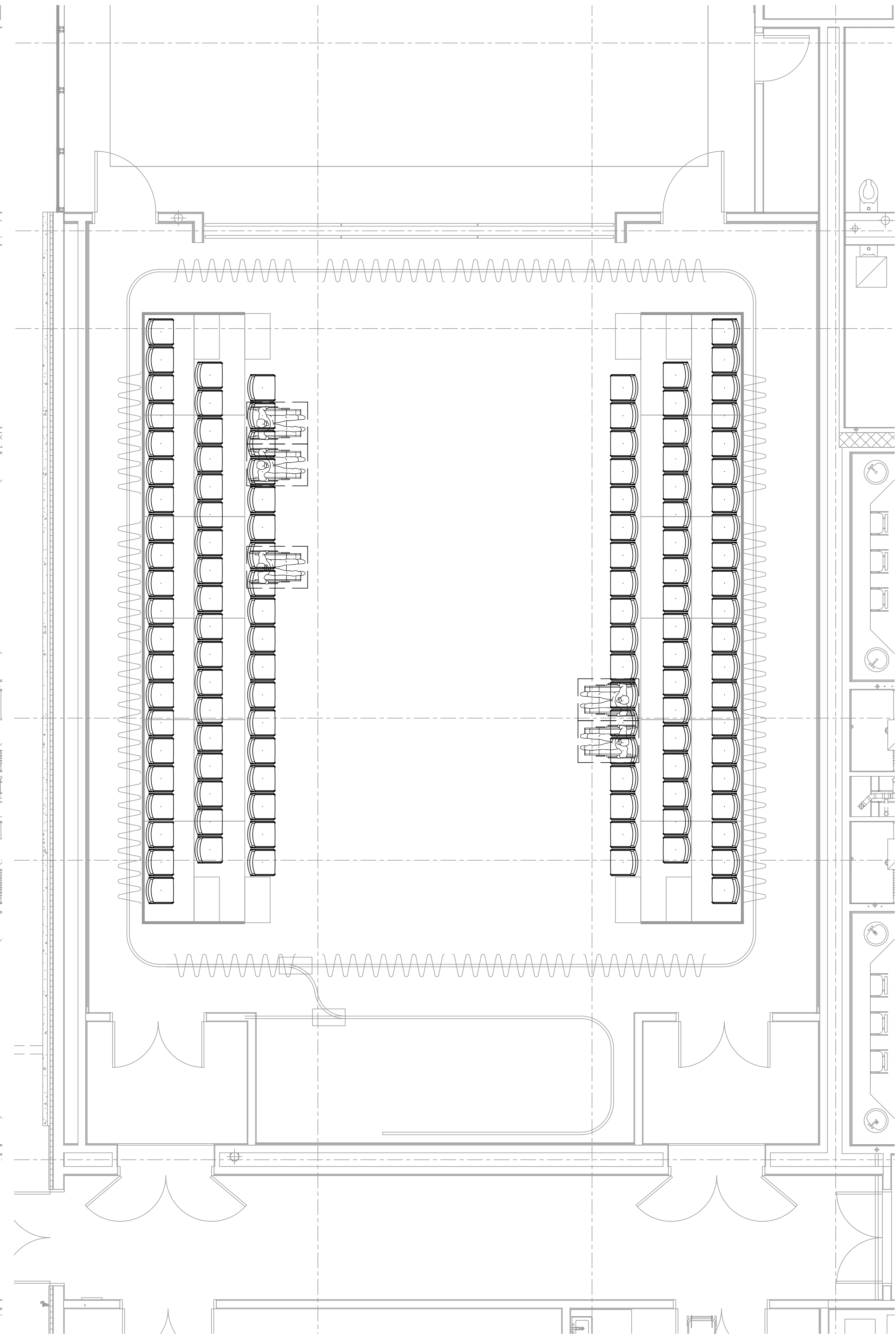
1 PLAN - STUDIO THEATRE - PROMENADE CONFIGURATION SCALE: 1/4" = 1'-0"
