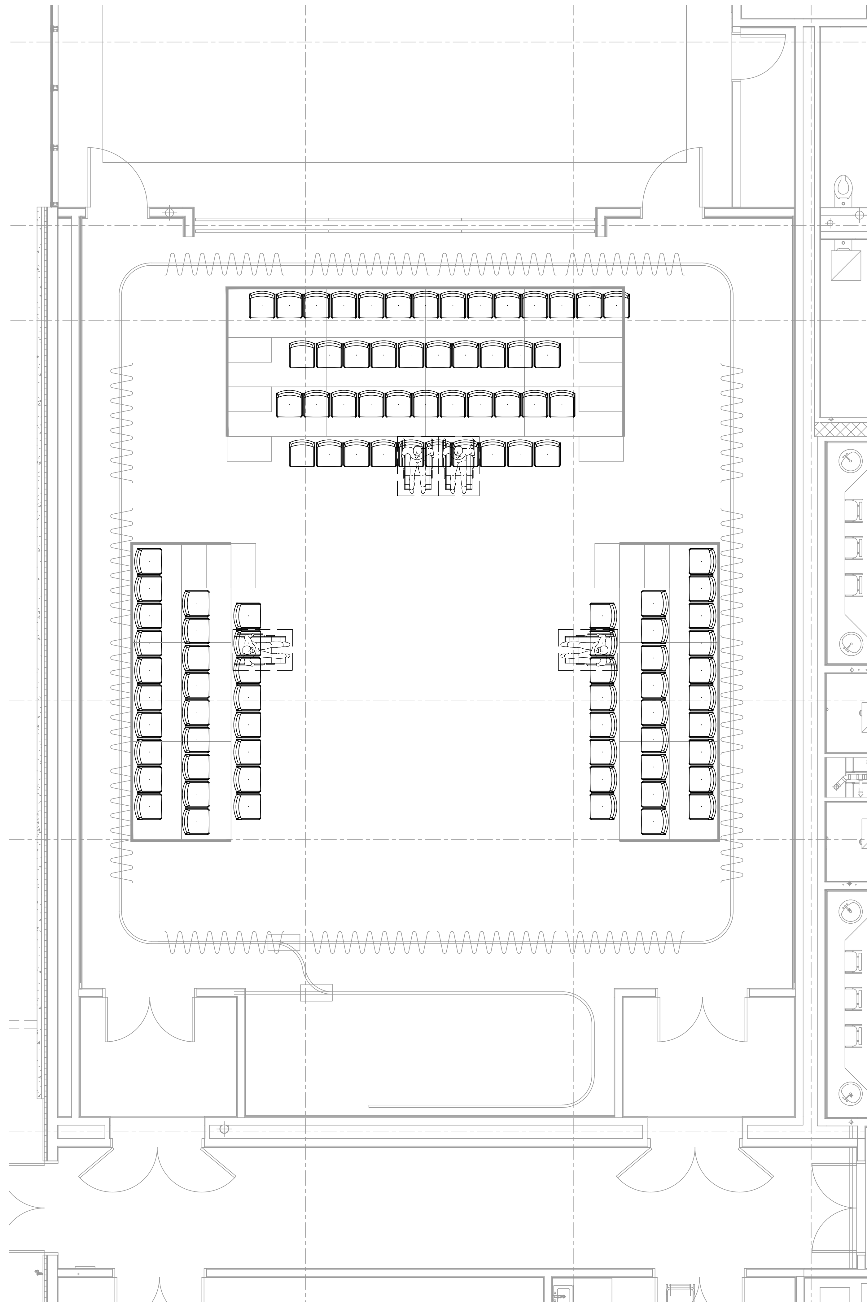
11 PLAN - STUDIO THEATRE - THRUST CONFIGURATION SCALE: 1/4" = 1'-0"
