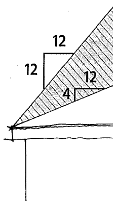
Figure 5: Roof and Eave Lines
