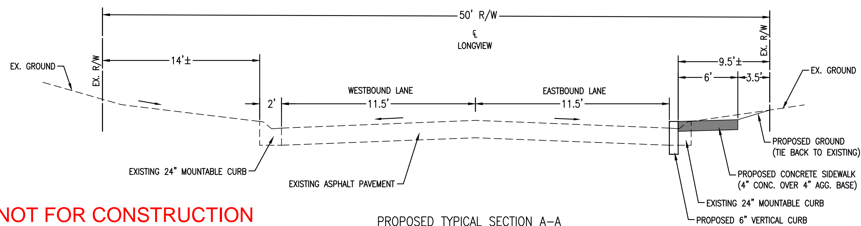
PROPOSED TYPICAL SECTION A-A
